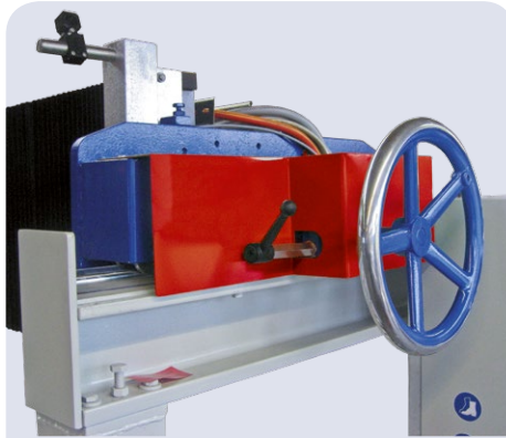
Side adjustment with digital readout (optional)
