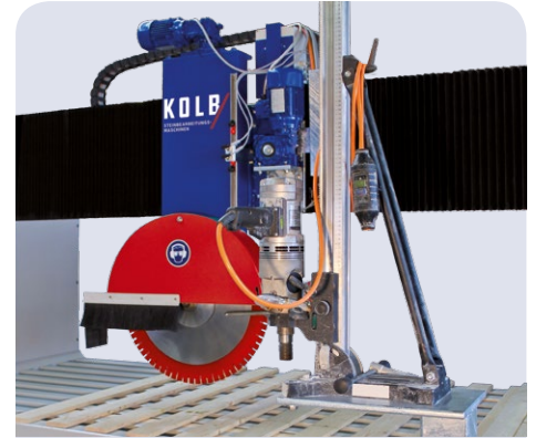
Drilling machine (optional)
